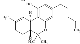
Tetrahydrocannabinol
