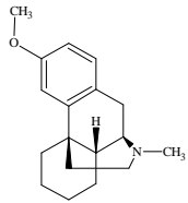
Dextromethorphan
