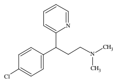
Chlorpheniramine
